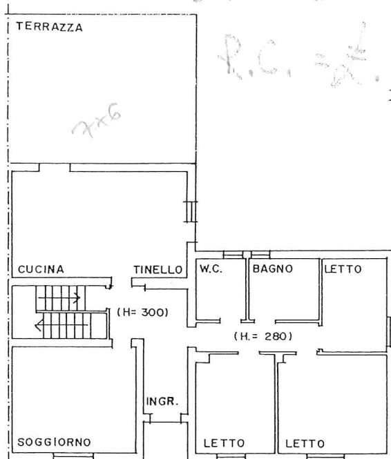
PIANO TERRA
